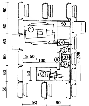
plan ① large projector ② diascope ③ Paradouit color Prado ④ 8 mm film projector ⑤ control panel
